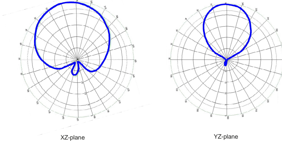
E-field elevation & Azimuth Patterns
